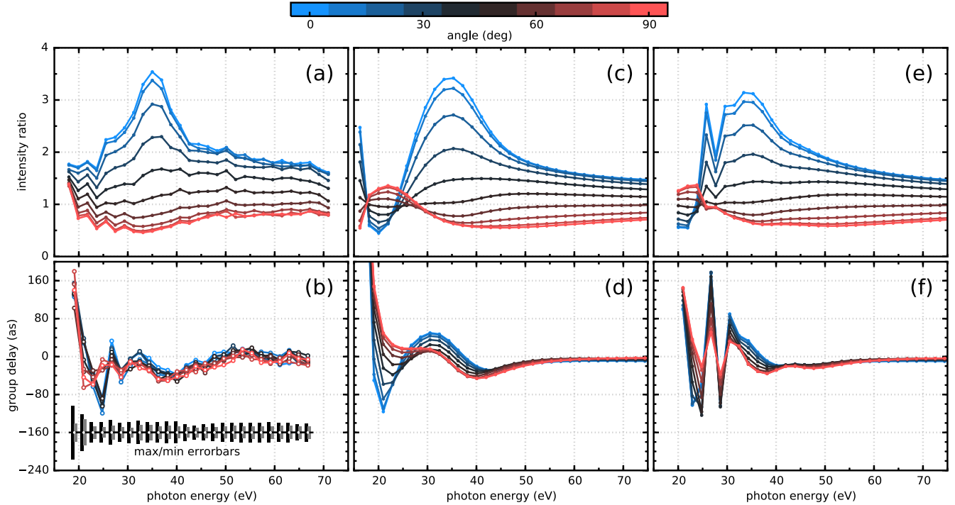
FIG. 3. Complex dipole of N_2 . Harmonic spectral intensity normalized to the isotropic yield for different alignment angles from 0^\circ (light blue) to 90^\circ (light red) as measured experimentally (a) and as predicted by theory using three- (c) and eight- (e) channel angle-convolved photoionization dipole moments. Dipole group delay as measured experimentally (b) and as predicted by theory using three (d) and eight (f) channels. In (b) only the largest and smallest error bars are shown and offset for clarity. The standard error of the experimental group delay is estimated from the fit to the RABBITT sideband oscillations.
