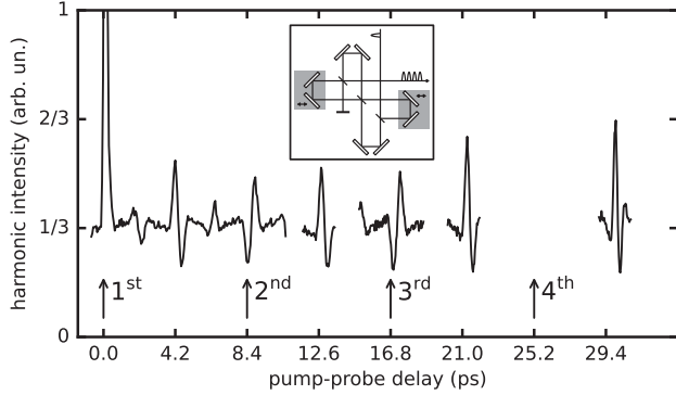
FIG. 1. HHG spectral intensity at 32 eV from N_2 as a function of the pump-probe delay. The inset shows the nested interferometer which creates the four-kicker pulse train used to populate a coherent rotational wave packet in the molecular ensemble. Each arrow indicates the delay of one kick. At 0 delay, the huge enhancement is due to the pump-probe temporal overlap. At 8.4 ps delay (respectively 16.8 ps), the trace was recorded in the absence of the second (third) kick.
