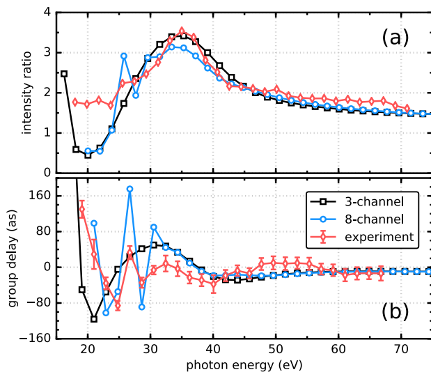
FIG. 4. Complex dipole of N 2 along the internuclear axis. Direct comparison between experiment and the three- and eight-channel model of the dipole normalized intensity (a) and group delay (b) for the ensemble of N 2 aligned at 0°.
