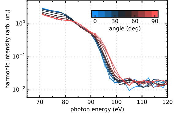
FIG. 2. N_2 harmonic spectral intensity in the cutoff region. Alignment angles are shown from 0^\circ (light blue) to 90^\circ (light red). Each harmonic order is integrated for clarity.
